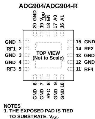
Figure 6. 20-Lead 4 mm × 4mm LFCSP (CP-20-6)
